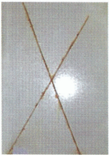
Steel Guard Coated Followed by single coat Epoxy Paint after 1200 Hours in Salt Spray Machine as per ASTM B-117
